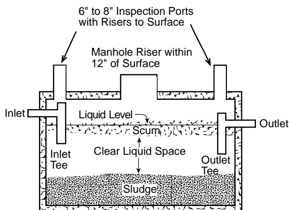
Septic Tank
